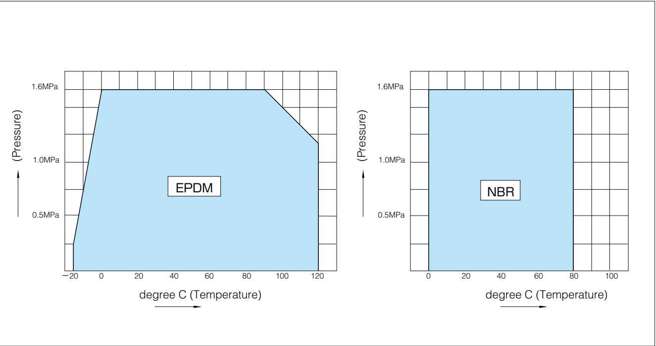
731P Pressure-temperature rating
